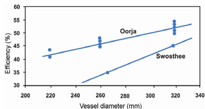
Figure 3. Effect of vessel diameter on efficiency, the lower plot is for the stove named Swosthee 4 .
