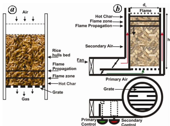
Figure 1. a , Schematic view of a rice hull gasifier. Note that the air flows from the open top towards the bottom. b , Schematic representation of a reverse downdraft gasifier stove where the gasification air flows from bottom to top.
