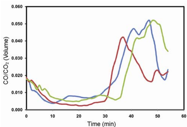
Figure 4. Variation of the volumetric ratio of CO:CO 2 during a stove operation. The operation till 30 min is in flaming mode; char mode operation begins after a short transition.
